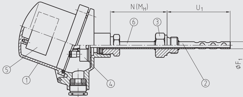
Fig. with parallel thread, for tapered thread see "Process connection"
